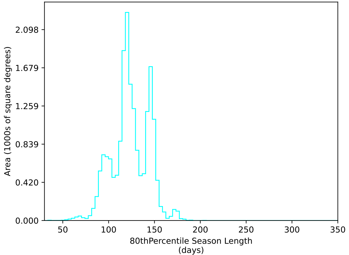
ddf_acor_sf20_lsf40_lsr10_v3.4_10yrs WFD u band: 80thPercentile Season Length
