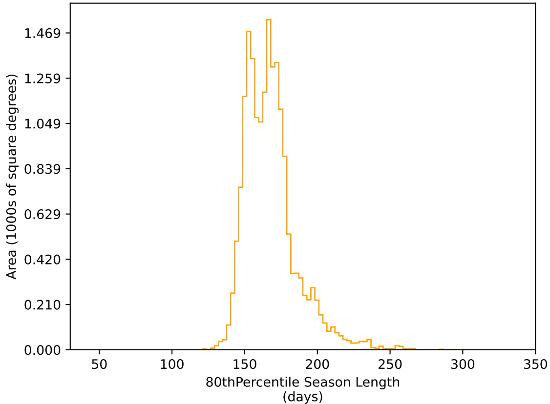
ddf_acor_sf20_lsf40_lsr10_v3.4_10yrs WFD r band: 80thPercentile Season Length
