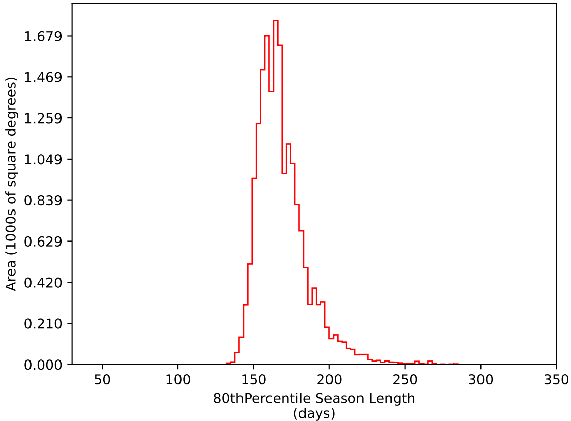
ddf_acor_sf20_lsf40_lsr10_v3.4_10yrs WFD i band: 80thPercentile Season Length
