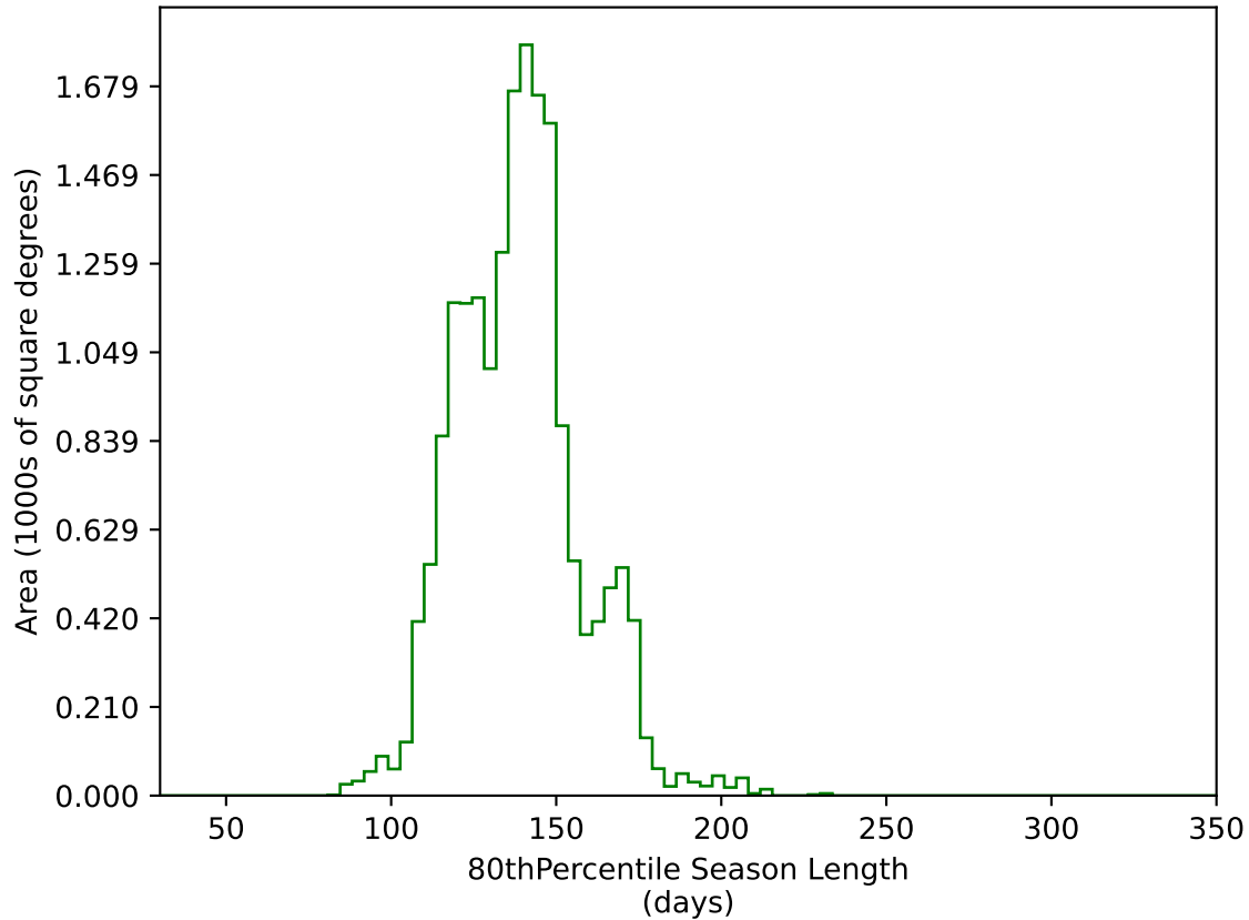
ddf_acor_sf20_lsf40_lsr10_v3.4_10yrs WFD g band: 80thPercentile Season Length
