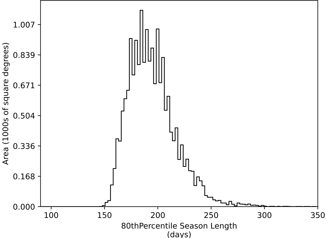
ddf_acor_sf20_lsf40_lsr10_v3.4_10yrs WFD all bands: 80thPercentile Season Length
