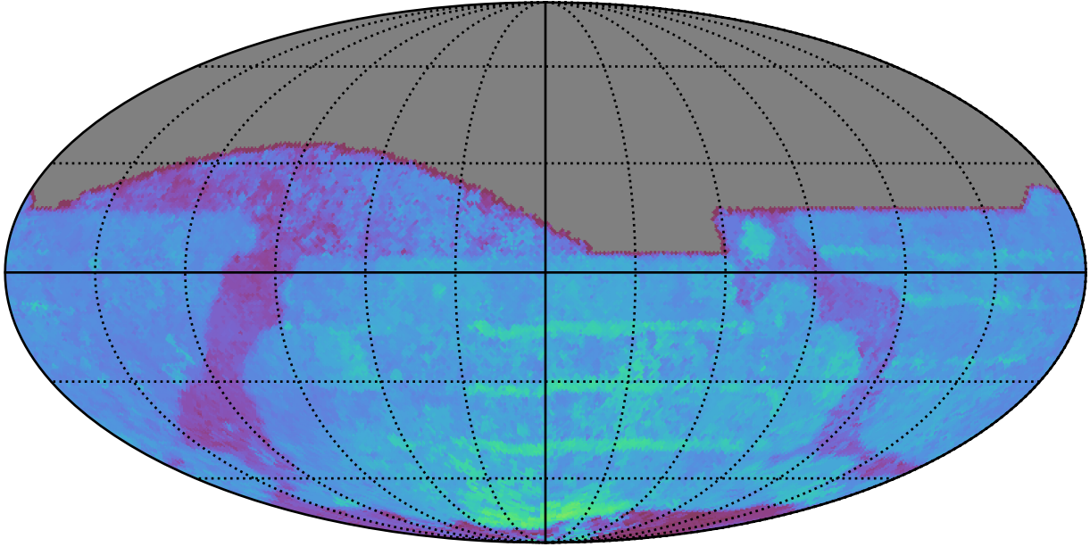
ddf_acor_sf20_lsf40_lsr10_v3.4_10yrs All sky z band: 80thPercentile Season Length
