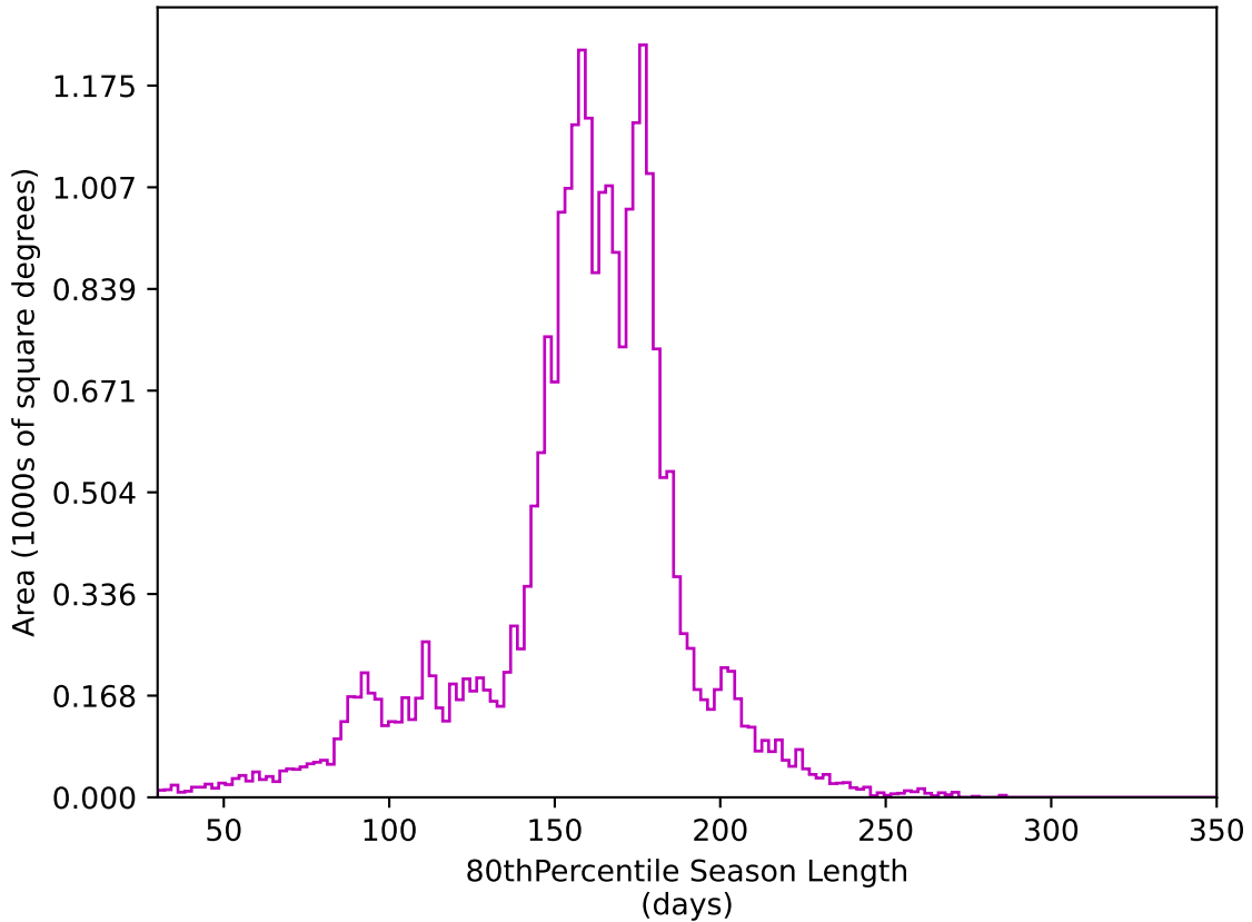
ddf_acor_sf20_lsf40_lsr10_v3.4_10yrs All sky z band: 80thPercentile Season Length
