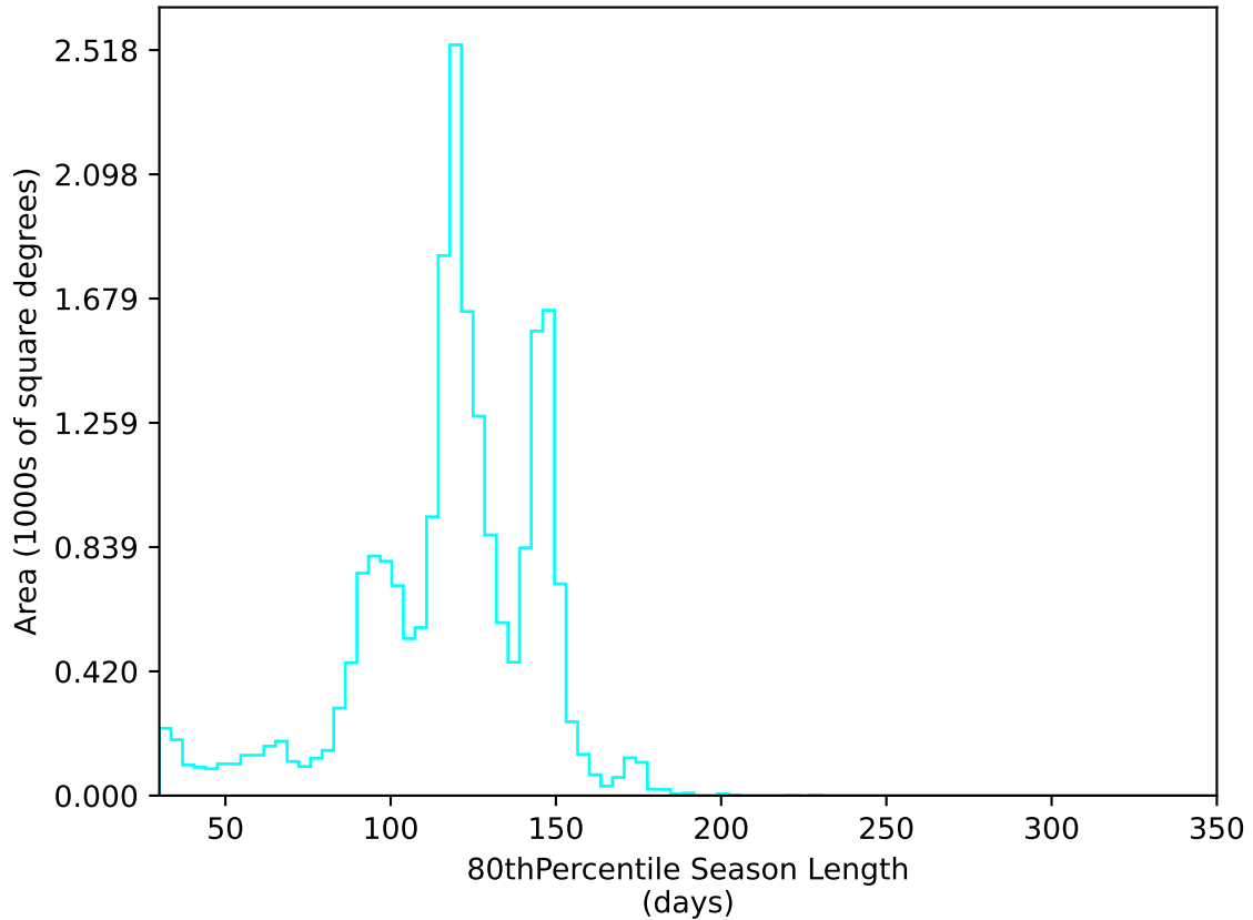
ddf_acor_sf20_lsf40_lsr10_v3.4_10yrs All sky u band: 80thPercentile Season Length
