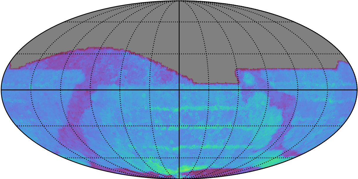
ddf_acor_sf20_lsf40_lsr10_v3.4_10yrs All sky r band: 80thPercentile Season Length
