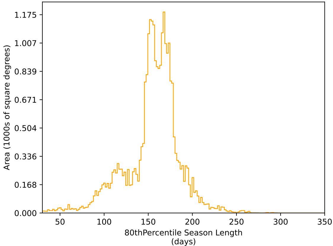
ddf_acor_sf20_lsf40_lsr10_v3.4_10yrs All sky r band: 80thPercentile Season Length
