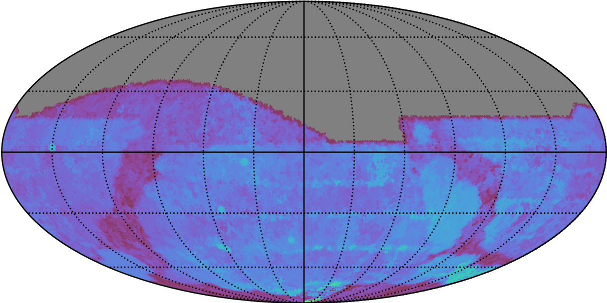
ddf_acor_sf20_lsf40_lsr10_v3.4_10yrs All sky g band: 80thPercentile Season Length
