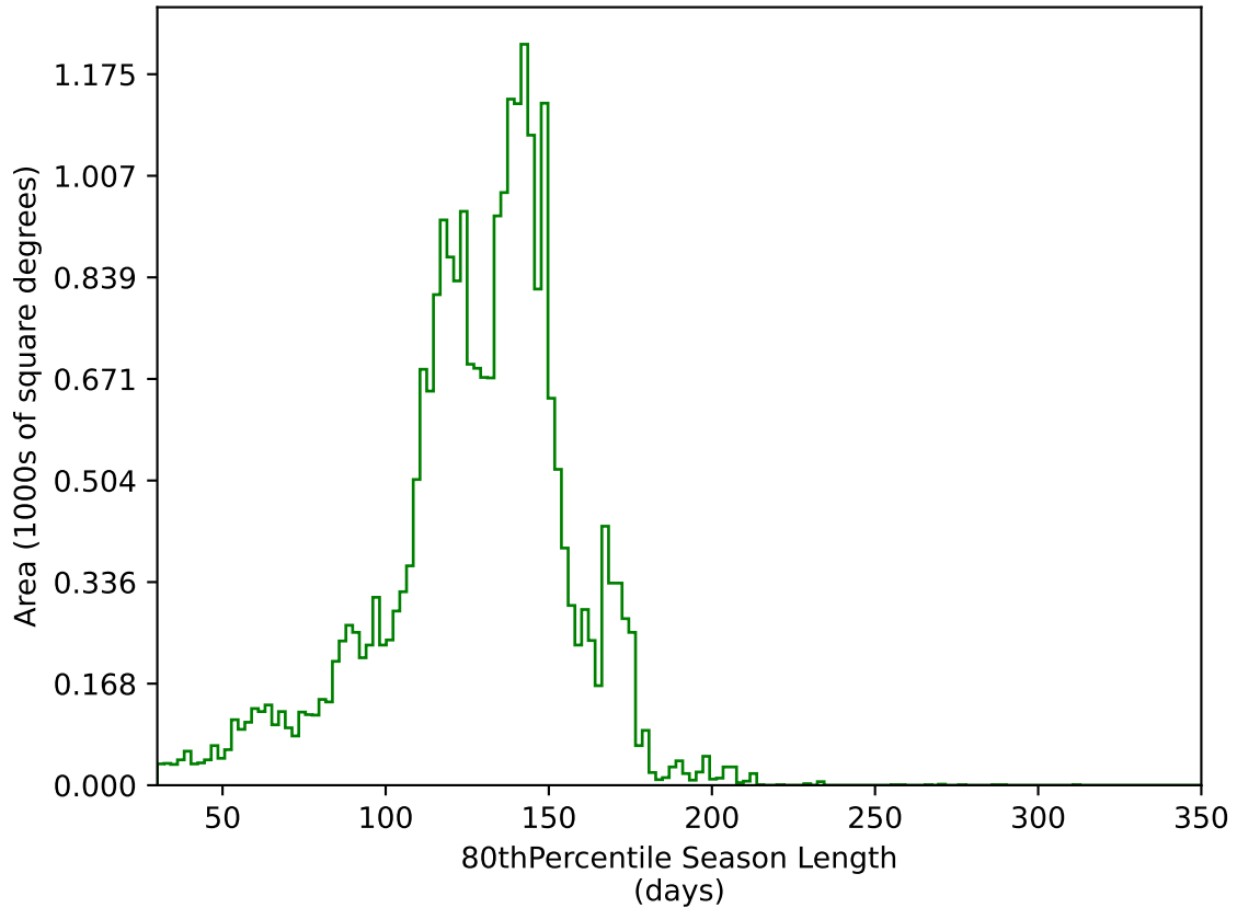
ddf_acor_sf20_lsf40_lsr10_v3.4_10yrs All sky g band: 80thPercentile Season Length
