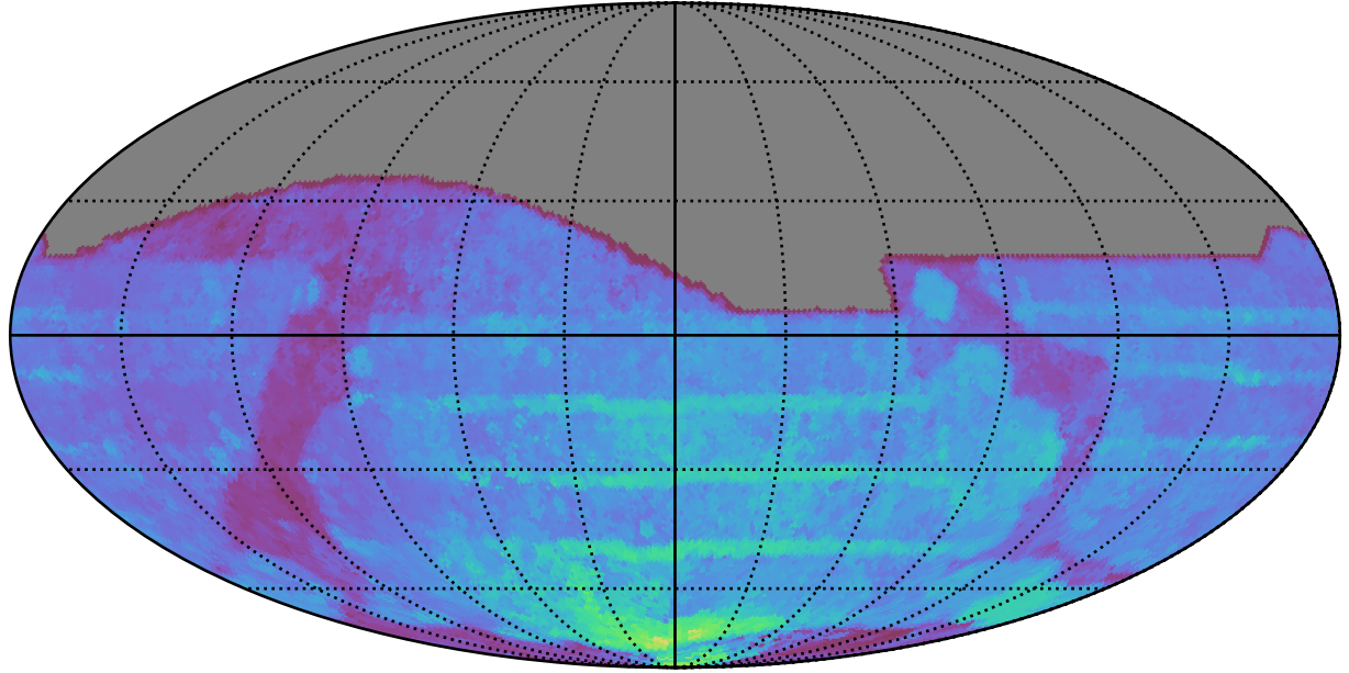
ddf_acor_sf20_lsf40_lsr10_v3.4_10yrs All sky all bands: 80thPercentile Season Length
