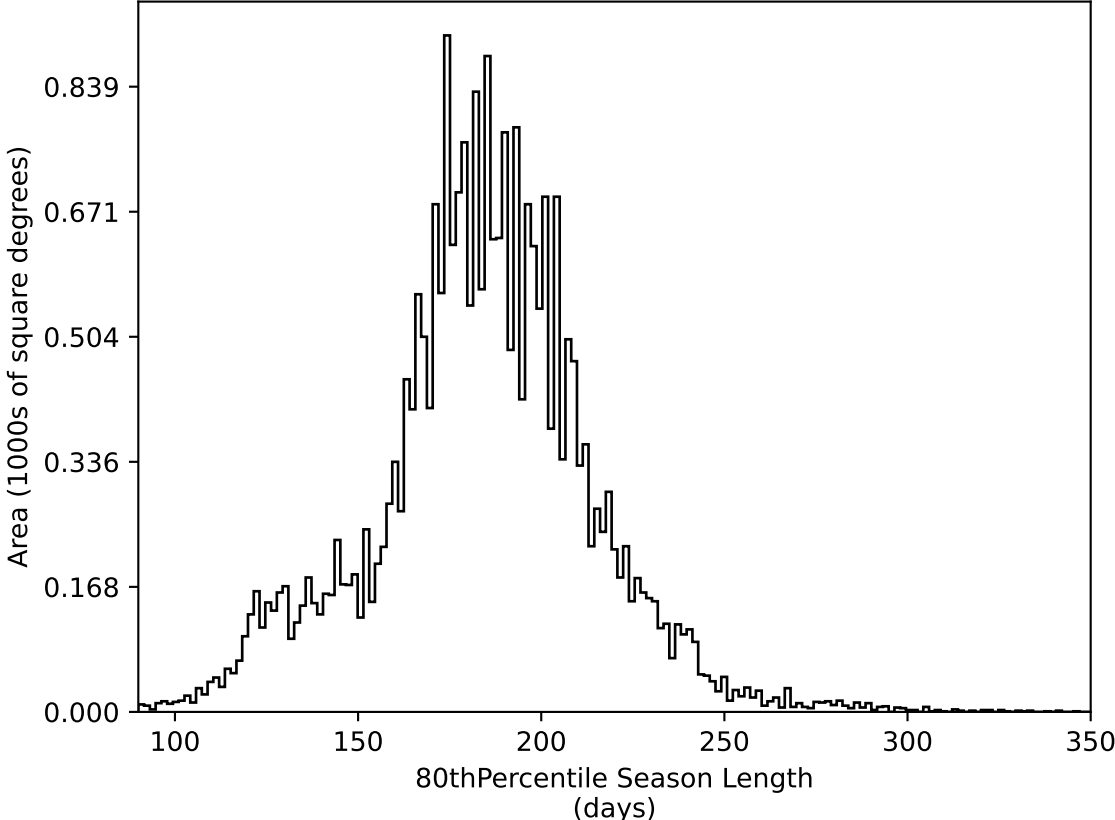
ddf_acor_sf20_lsf40_lsr10_v3.4_10yrs All sky all bands: 80thPercentile Season Length
