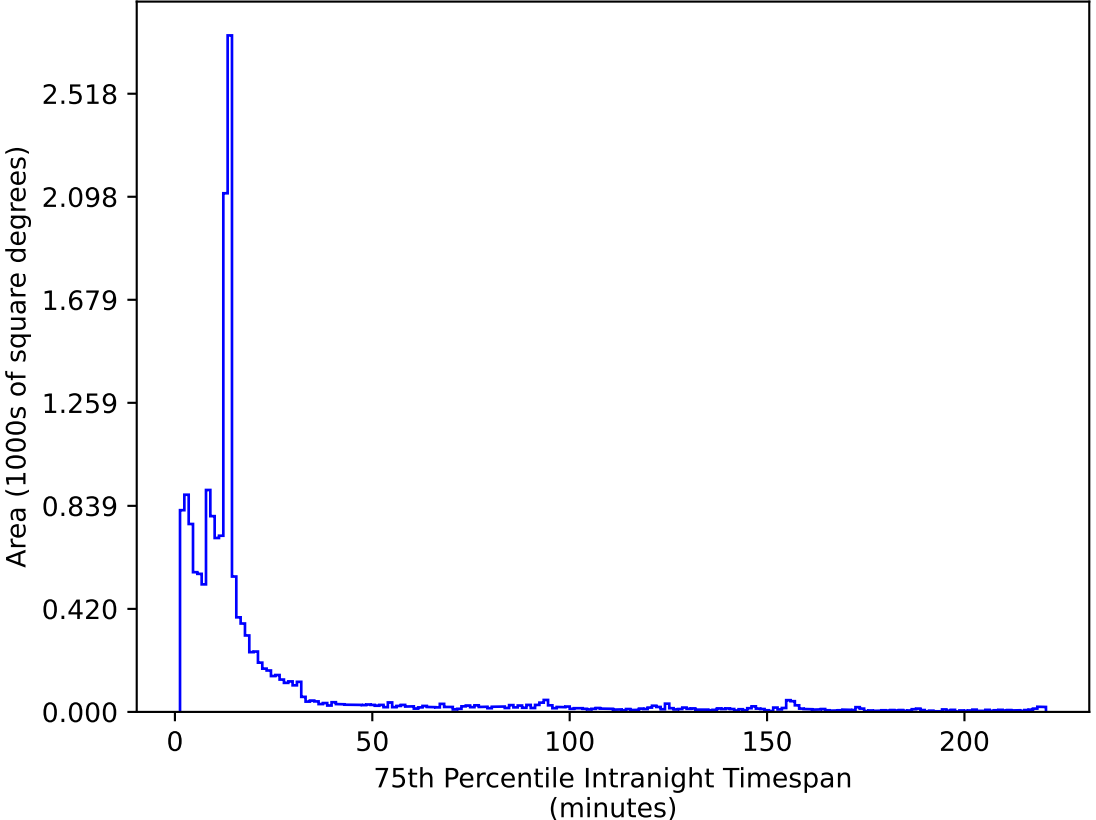
ddf_acor_sf20_lsf40_lsr10_v3.4_10yrs WFD z band: 75th Percentile Intranight Timespan
