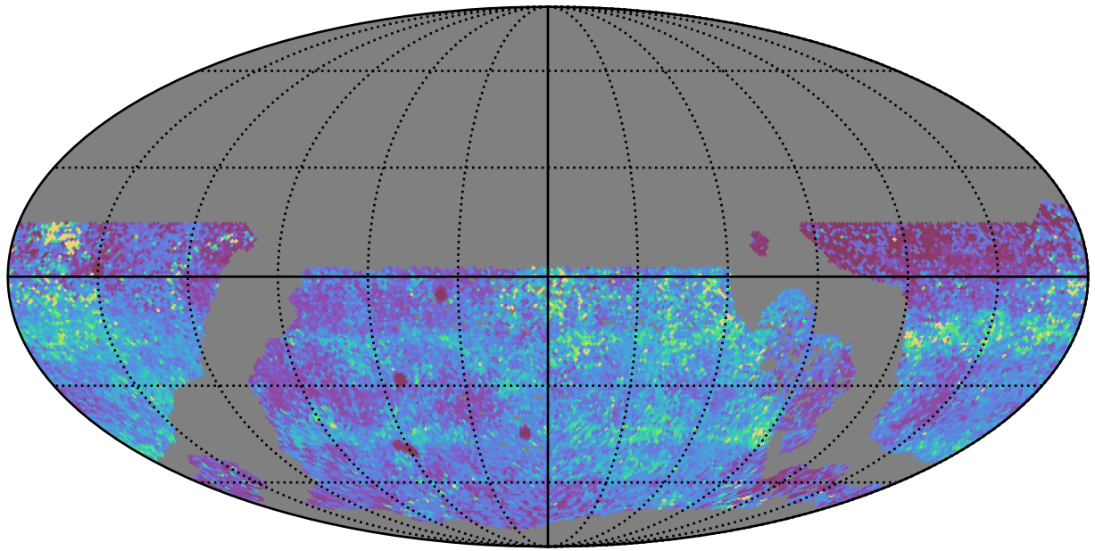
ddf_acor_sf20_lsr40_lsr10_v3.4_10yrs WFD y band: 75th Percentile Intranight Timespan
