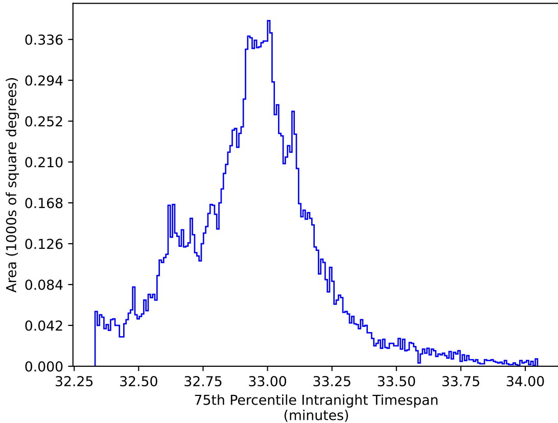
ddf_acor_sf20_lsf40_lsr10_v3.4_10yrs WFD y band: 75th Percentile Intranight Timespan
