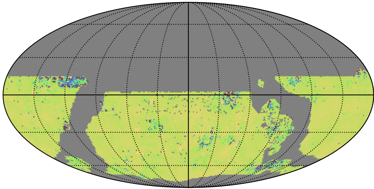
ddf_acor_sf20_lsf40_lsr10_v3.4_10yrs WFD ug bands: 75th Percentile Intranight Timespan
