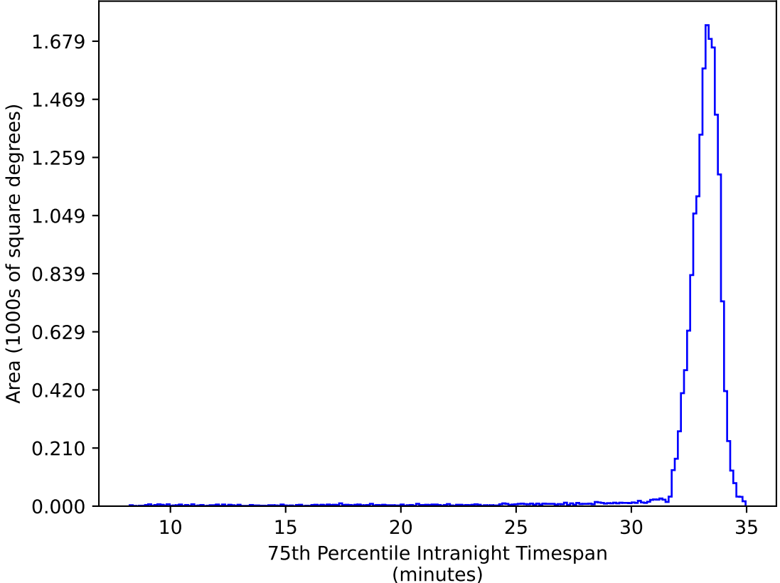
ddf_acor_sf20_lsf40_lsr10_v3.4_10yrs WFD ug bands: 75th Percentile Intranight Timespan
