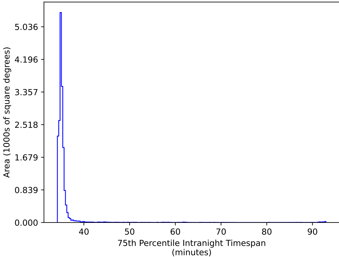
ddf_acor_sf20_lsf40_lsr10_v3.4_10yrs WFD ri bands: 75th Percentile Intranight Timespan
