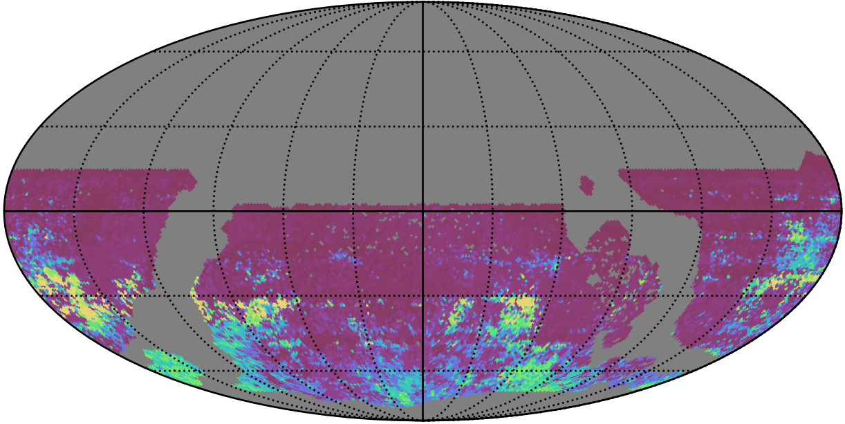
ddf_acor_sf20_lsf40_lsr10_v3.4_10yrs WFD r band: 75th Percentile Intranight Timespan
