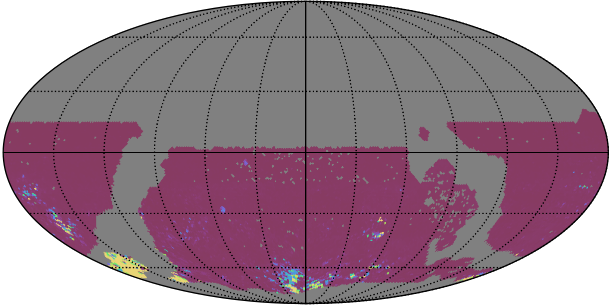
ddf_acor_sf20_lsf40_lsr10_v3.4_10yrs WFD gr bands: 75th Percentile Intranight Timespan
