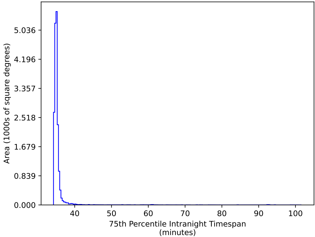
ddf_acor_sf20_lsf40_lsr10_v3.4_10yrs WFD gr bands: 75th Percentile Intranight Timespan
