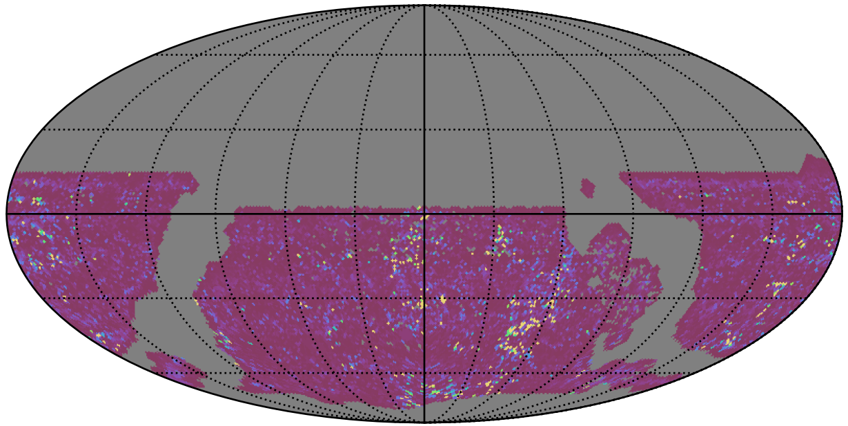
ddf_acor_sf20_lsf40_lsr10_v3.4_10yrs WFD g band: 75th Percentile Intranight Timespan
