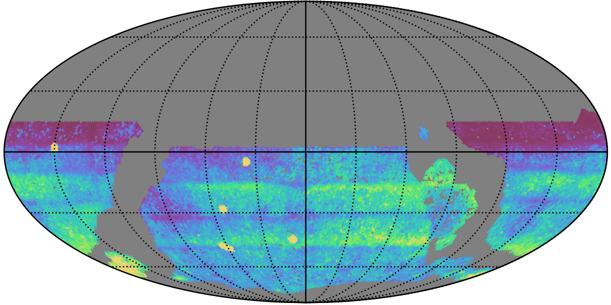
ddf_acor_sf20_lsf40_lsr10_v3.4_10yrs WFD all bands: 75th Percentile Intranight Timespan
