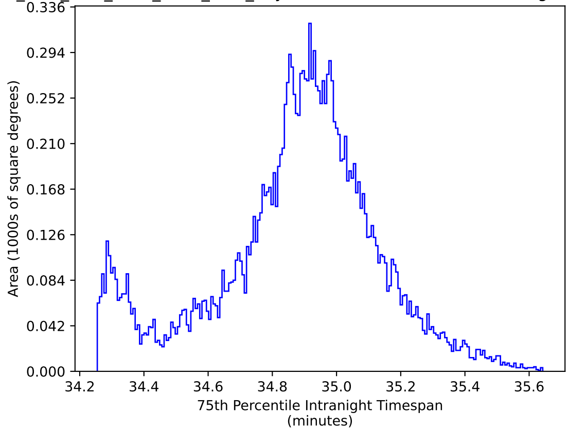
ddf_acor_sf20_lsf40_lsr10_v3.4_10yrs WFD: 75th Percentile Intranight Timespan
