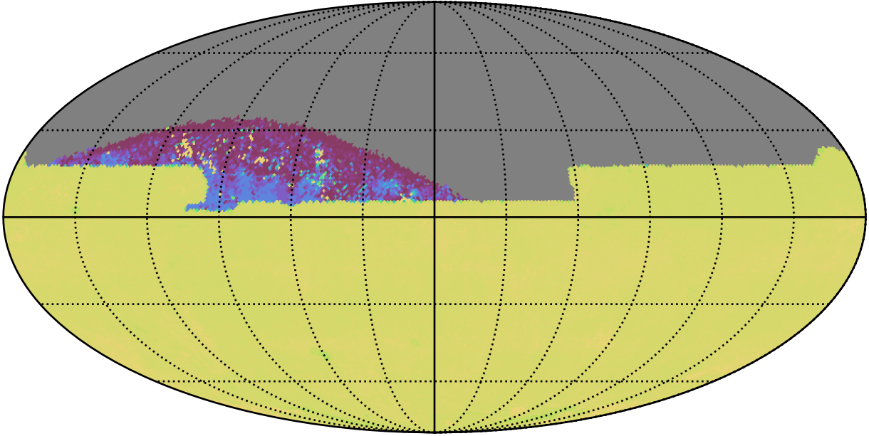
ddf_acor_sf20_lsf40_lsr10_v3.4_10yrs All sky zy bands: 75th Percentile Intranight Timespan
