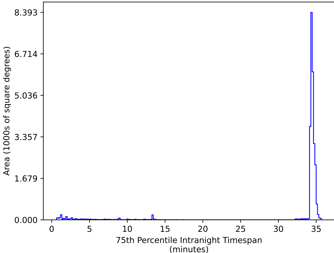
ddf_acor_sf20_lsf40_lsr10_v3.4_10yrs All sky zy bands: 75th Percentile Intranight Timespan
