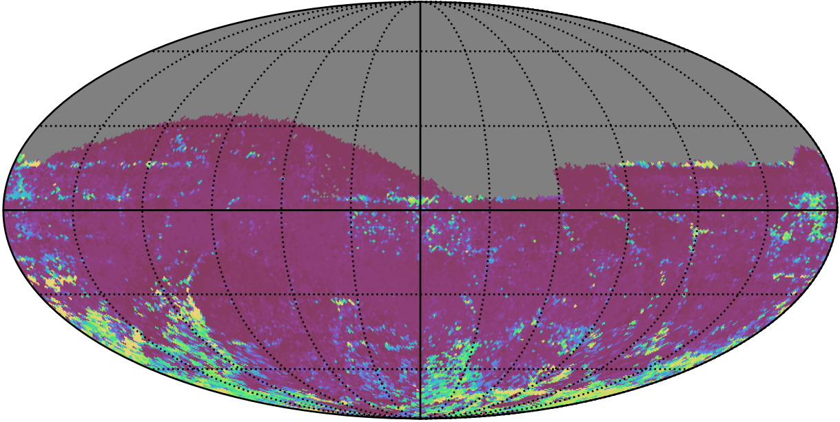
ddf_acor_sf20_lsf40_lsr10_v3.4_10yrs All sky z band: 75th Percentile Intranight Timespan
