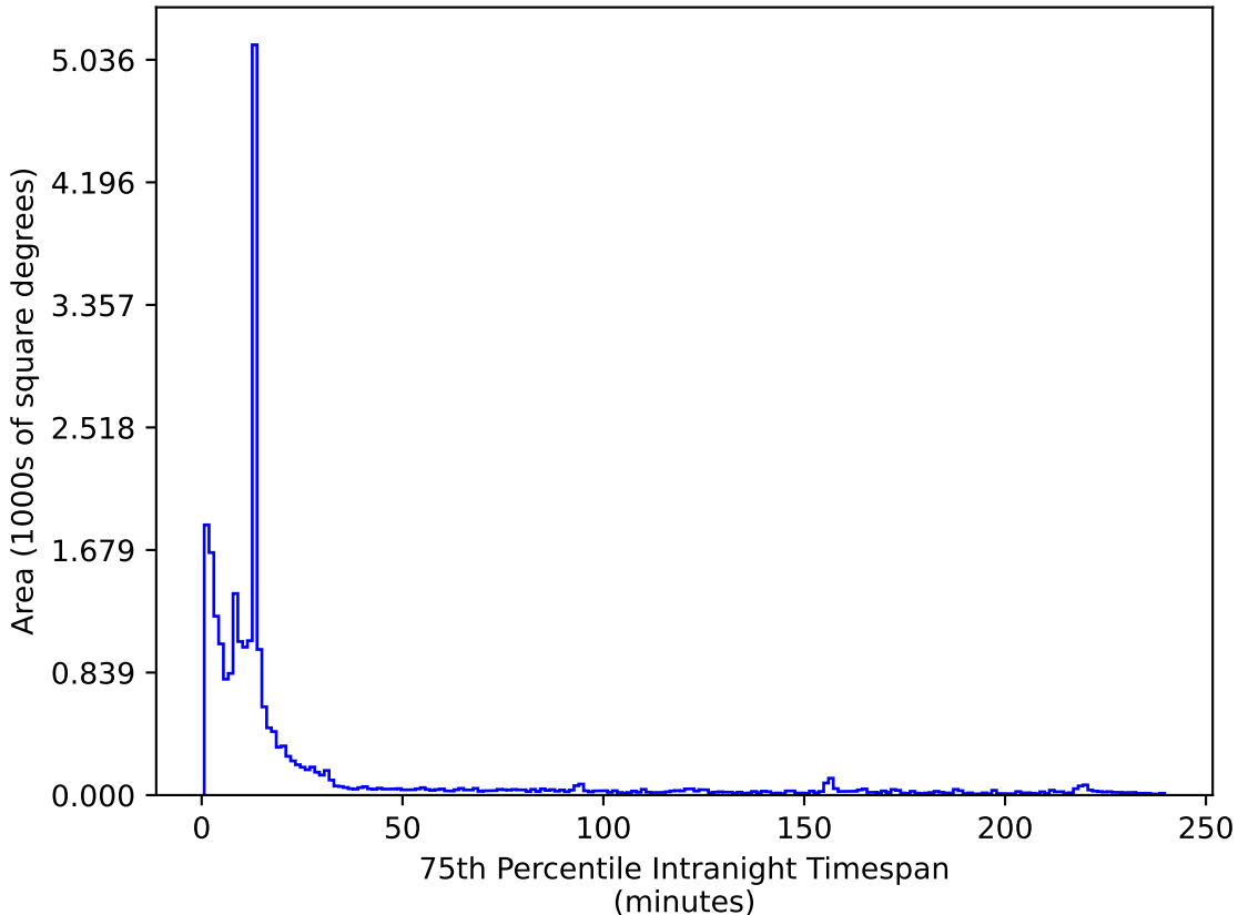
ddf_acor_sf20_lsf40_lsr10_v3.4_10yrs All sky z band: 75th Percentile Intranight Timespan
