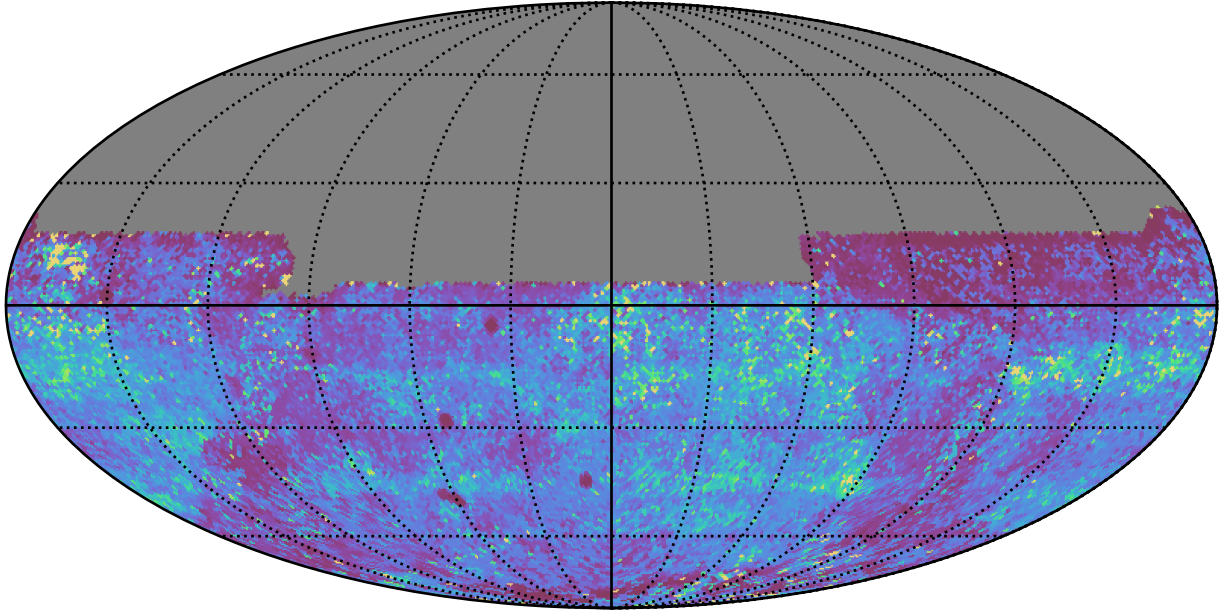
ddf_acor_sf20_lsf40_lsr10_v3.4_10yrs All sky y band: 75th Percentile Intranight Timespan
