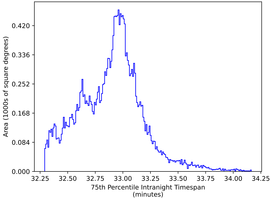
ddf_acor_sf20_lsf40_lsr10_v3.4_10yrs All sky y band: 75th Percentile Intranight Timespan
