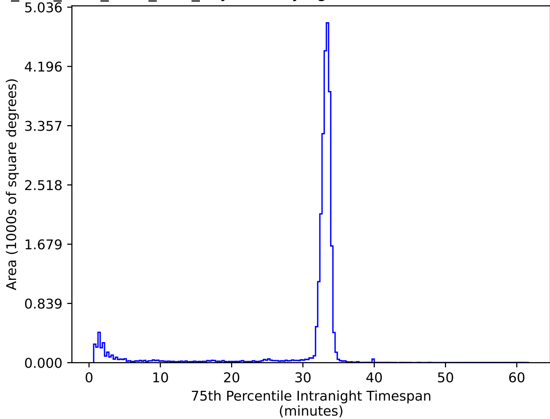
ddf_acor_sf20_lsf40_lsr10_v3.4_10yrs All sky ug bands: 75th Percentile Intranight Timespan
