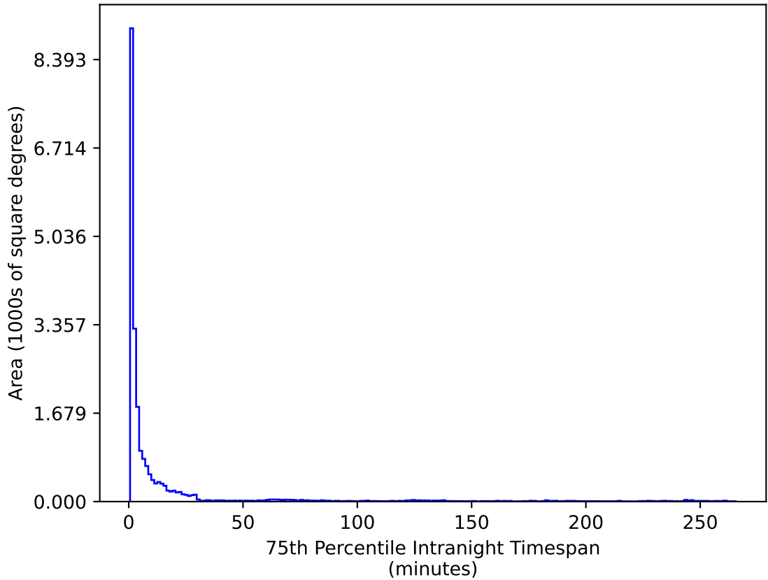
ddf_acor_sf20_lsf40_lsr10_v3.4_10yrs All sky u band: 75th Percentile Intranight Timespan
