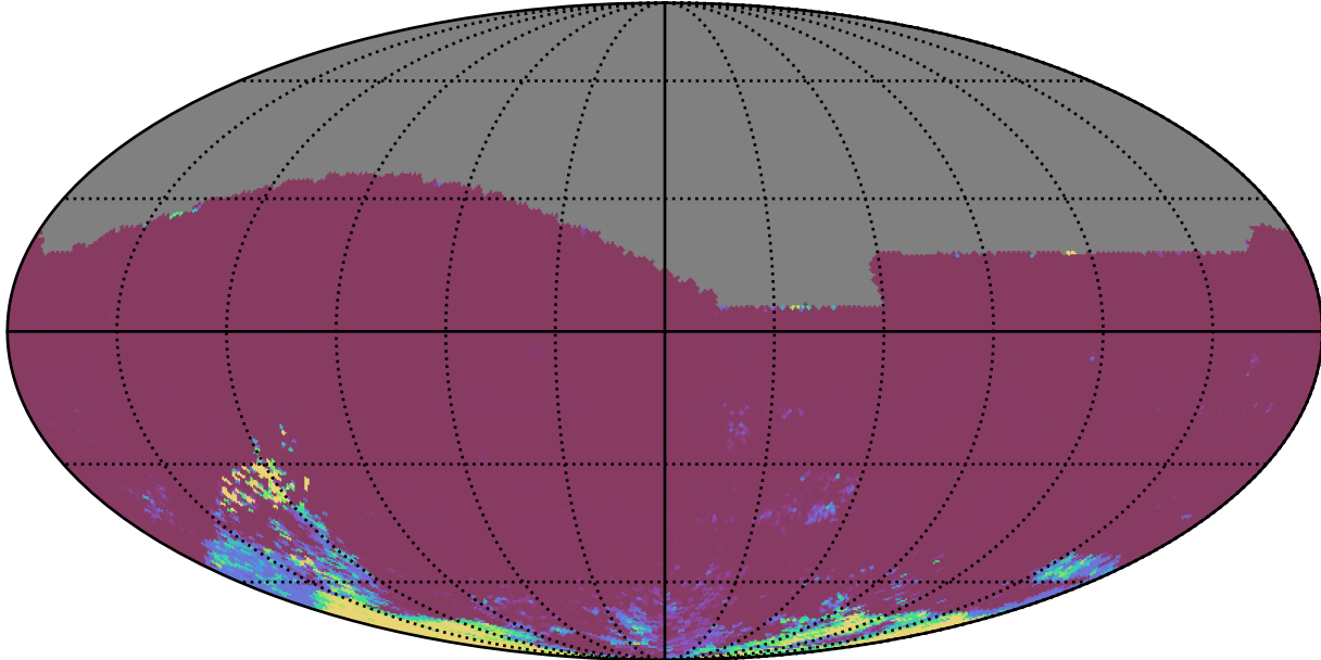
ddf_acor_sf20_lsf40_lsr10_v3.4_10yrs All sky ri bands: 75th Percentile Intranight Timespan
