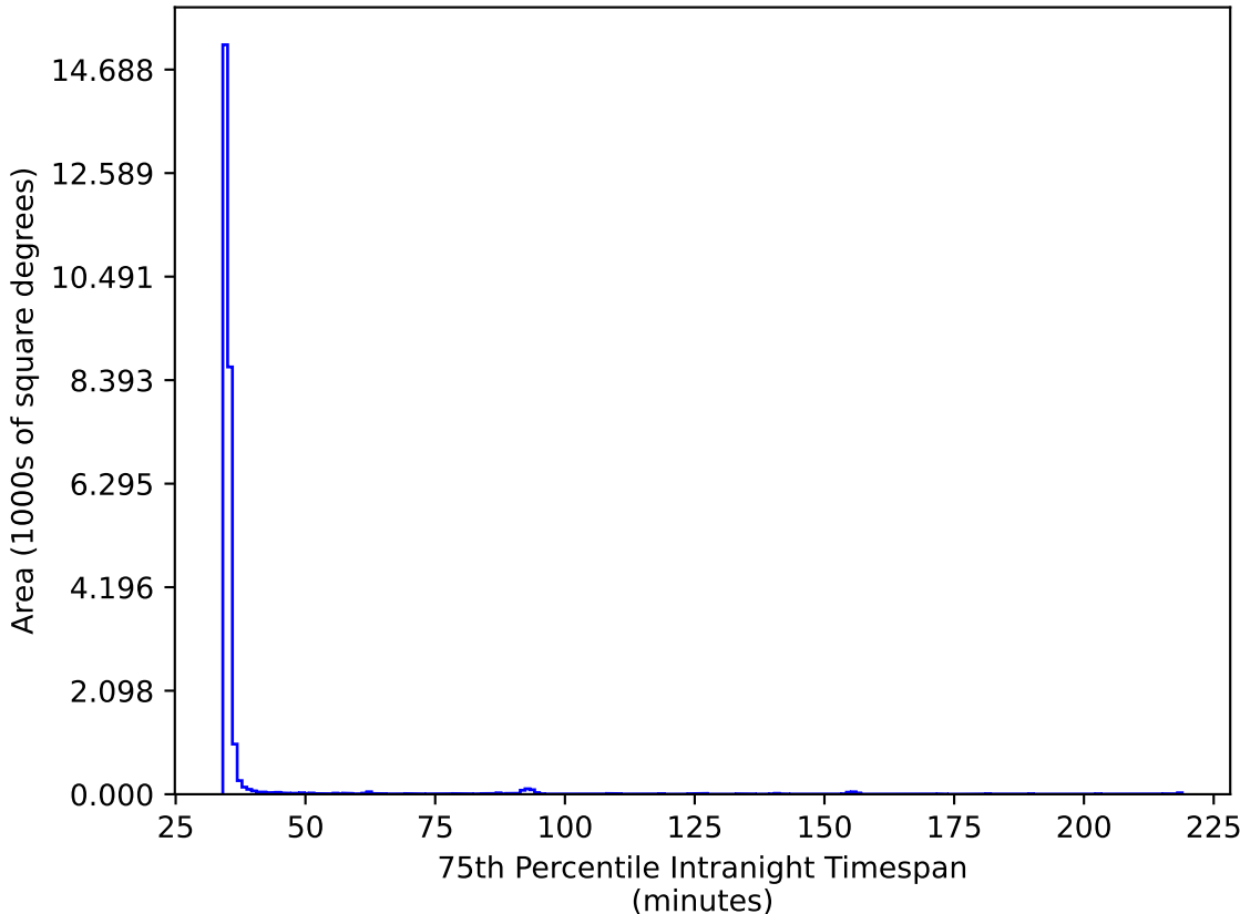
ddf_acor_sf20_lsf40_lsr10_v3.4_10yrs All sky ri bands: 75th Percentile Intranight Timespan
