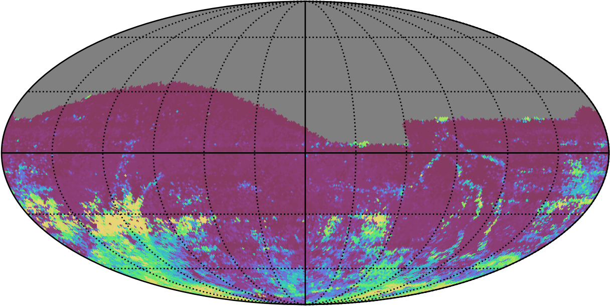
ddf_acor_sf20_lsf40_lsr10_v3.4_10yrs All sky r band: 75th Percentile Intranight Timespan
