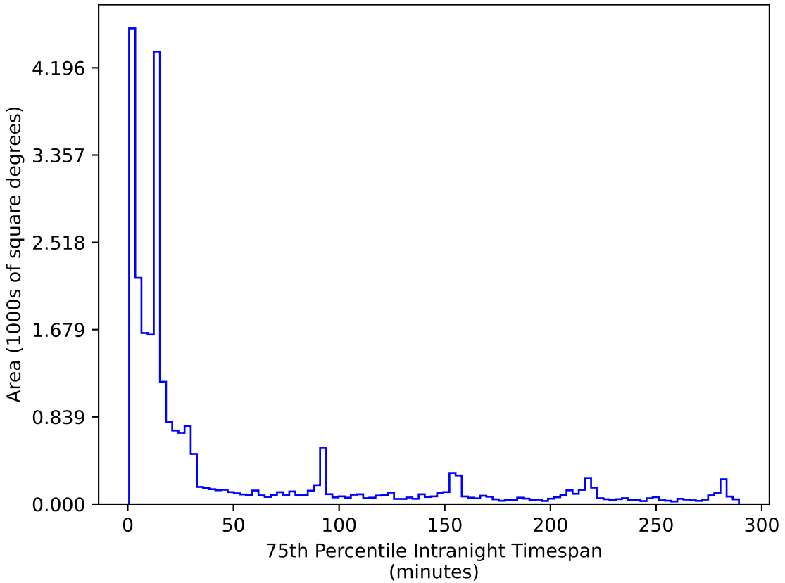
ddf_acor_sf20_lsf40_lsr10_v3.4_10yrs All sky r band: 75th Percentile Intranight Timespan
