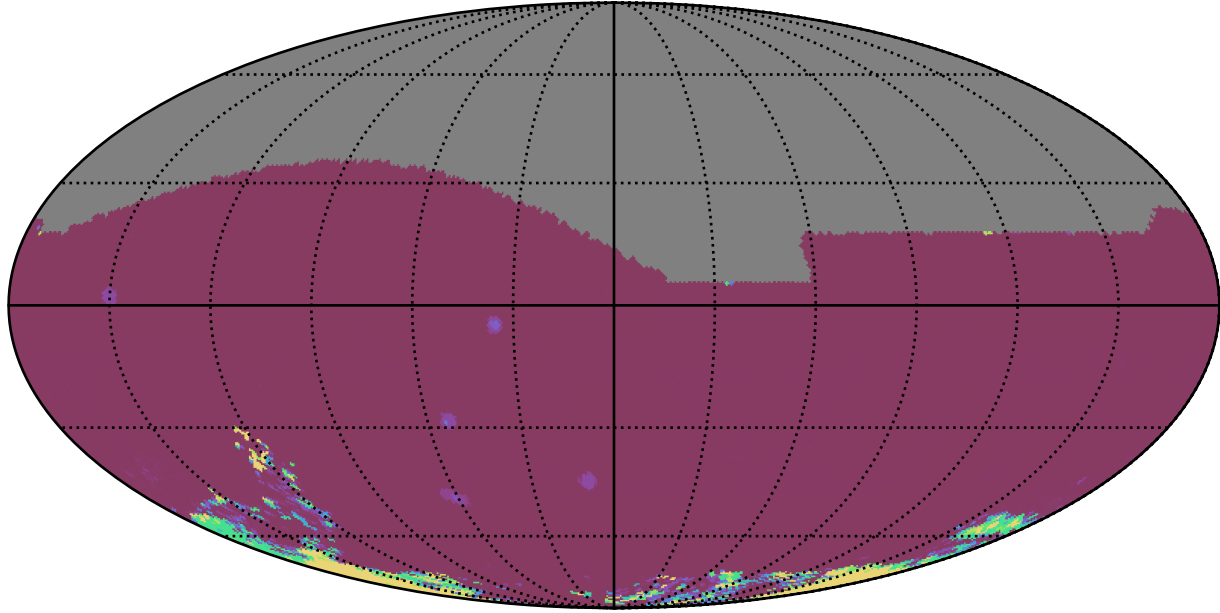
ddf_acor_sf20_lsf40_lsr10_v3.4_10yrs All sky iz bands: 75th Percentile Intranight Timespan
