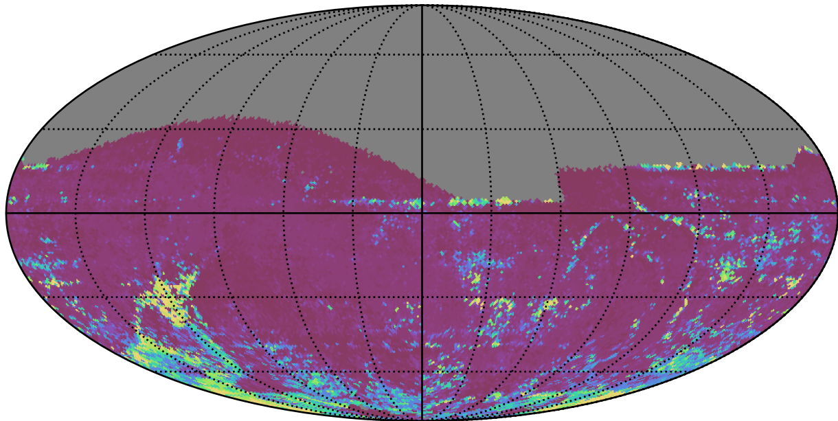
ddf_acor_sf20_lsf40_lsr10_v3.4_10yrs All sky i band: 75th Percentile Intranight Timespan
