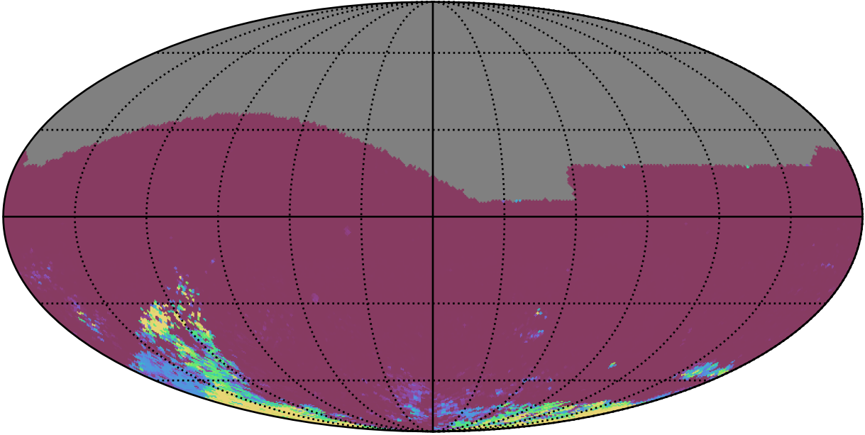
ddf_acor_sf20_lsf40_lsr10_v3.4_10yrs All sky gr bands: 75th Percentile Intranight Timespan
