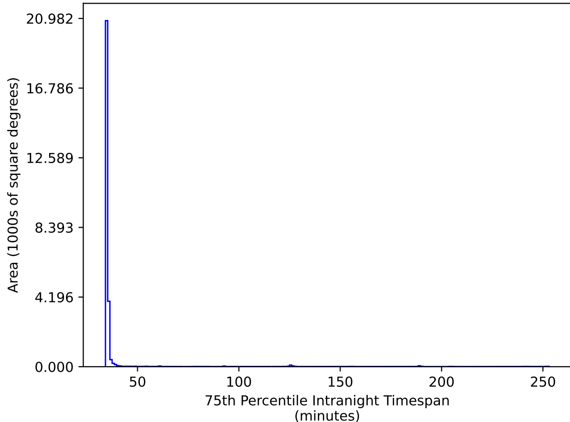
ddf_acor_sf20_lsf40_lsr10_v3.4_10yrs All sky gr bands: 75th Percentile Intranight Timespan
