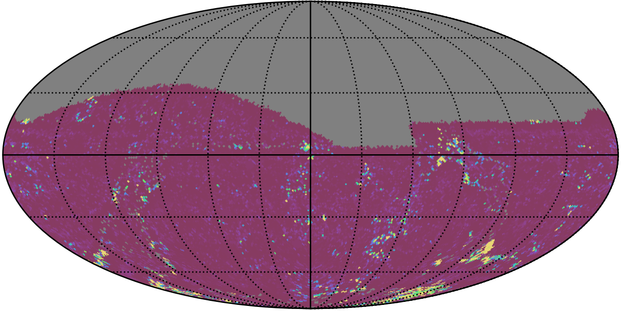
ddf_acor_sf20_lsf40_lsr10_v3.4_10yrs All sky g band: 75th Percentile Intranight Timespan
