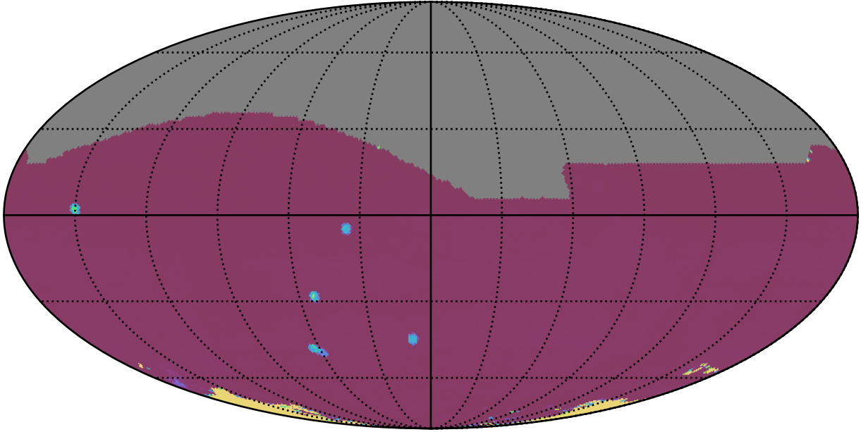
ddf_acor_sf20_lsf40_lsr10_v3.4_10yrs All sky all bands: 75th Percentile Intranight Timespan
