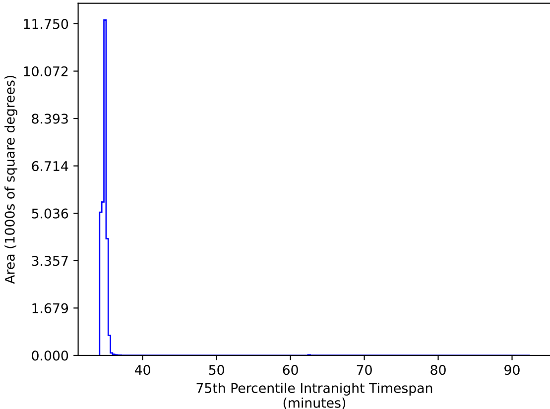
ddf_acor_sf20_lsf40_lsr10_v3.4_10yrs All sky all bands: 75th Percentile Intranight Timespan
