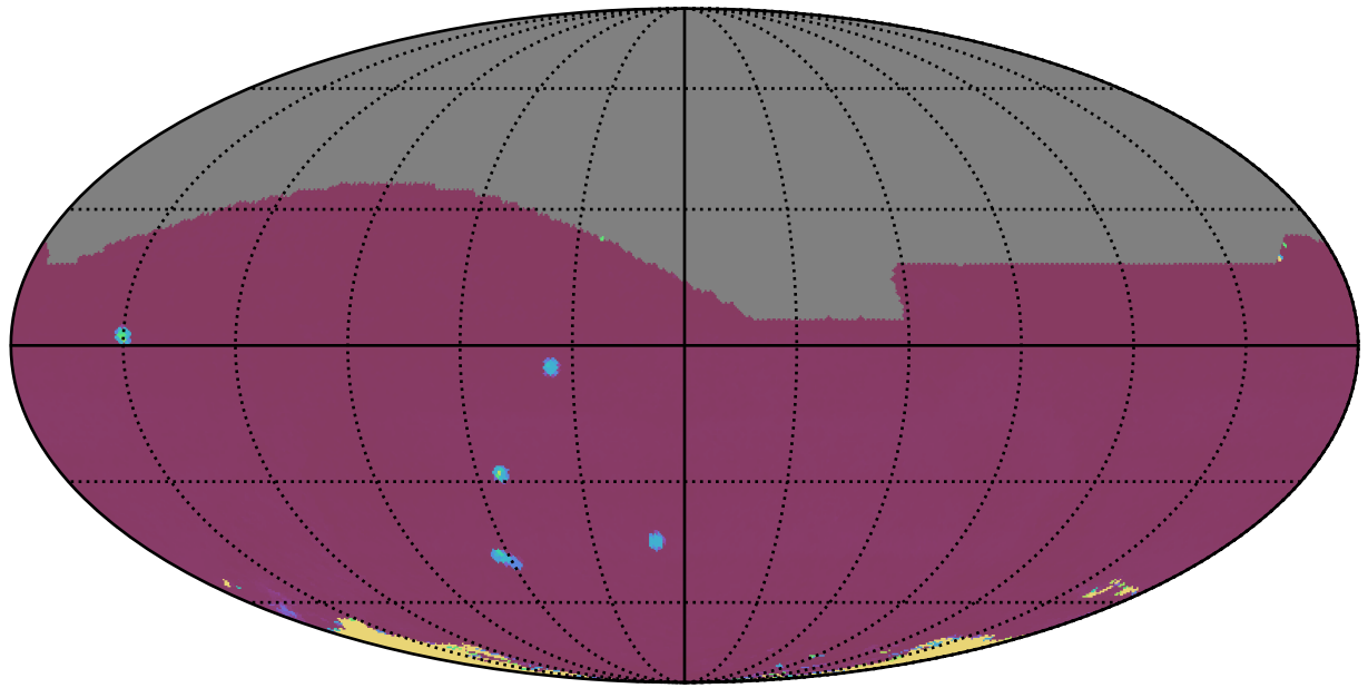
ddf_acor_sf20_lsf40_lsr10_v3.4_10yrs All sky: 75th Percentile Intranight Timespan
