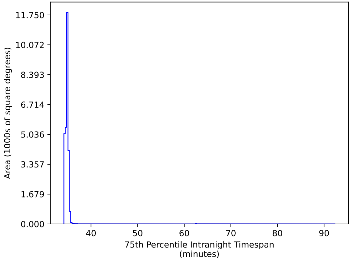
ddf_acor_sf20_lsf40_lsr10_v3.4_10yrs All sky: 75th Percentile Intranight Timespan
