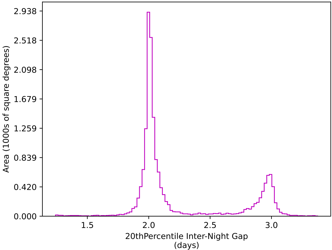
ddf_acor_sf20_lsf40_lsr10_v3.4_10yrs WFD z band: 20thPercentile Inter-Night Gap
