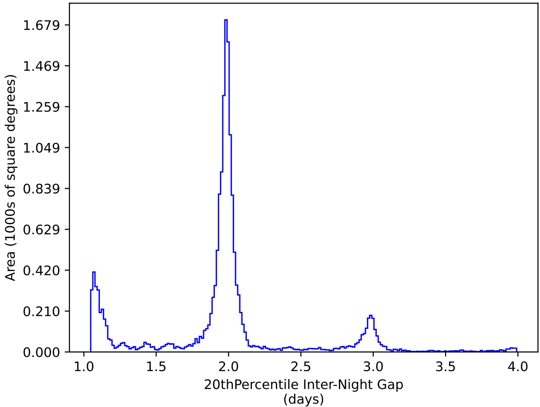
ddf_acor_sf20_lsf40_lsr10_v3.4_10yrs WFD y band: 20thPercentile Inter-Night Gap
