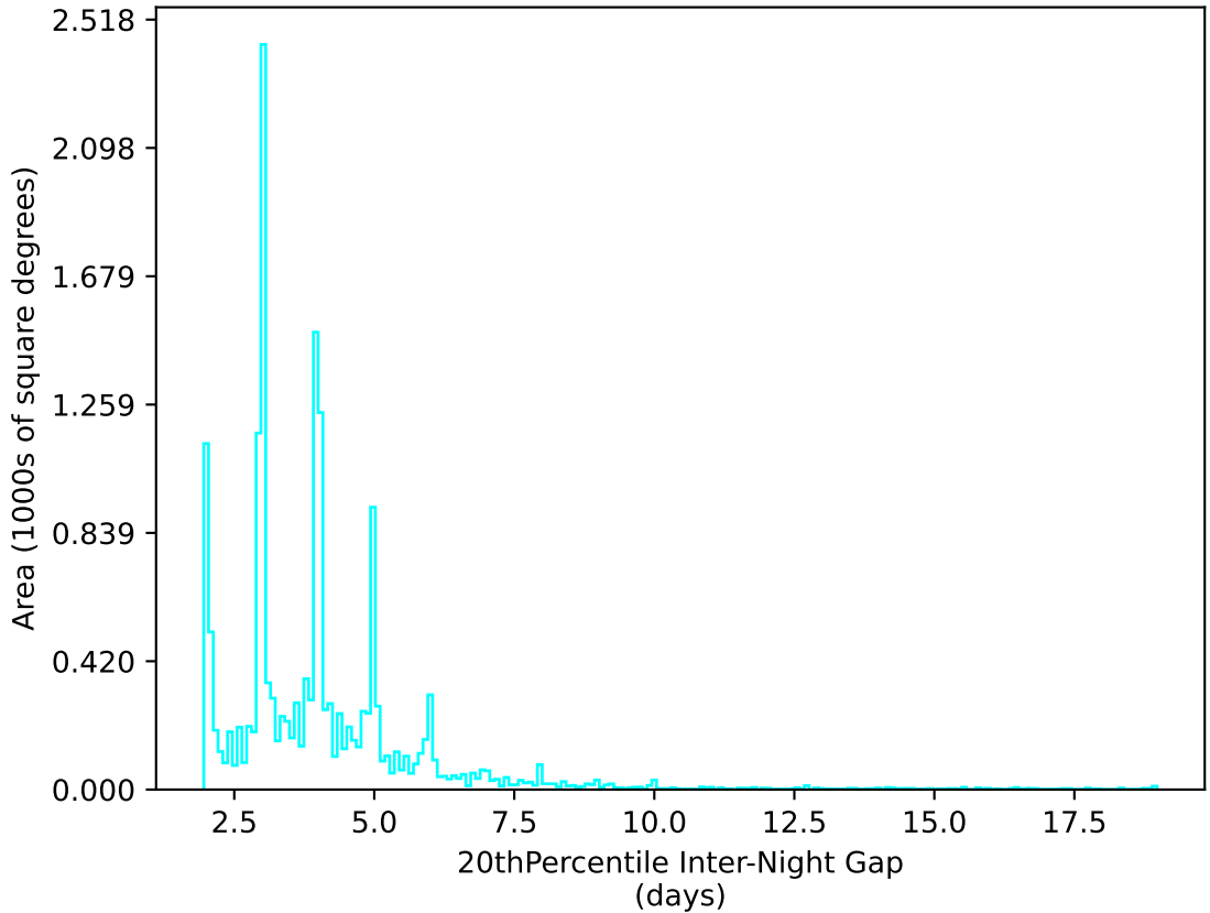
ddf_acor_sf20_lsf40_lsr10_v3.4_10yrs WFD u band: 20thPercentile Inter-Night Gap
